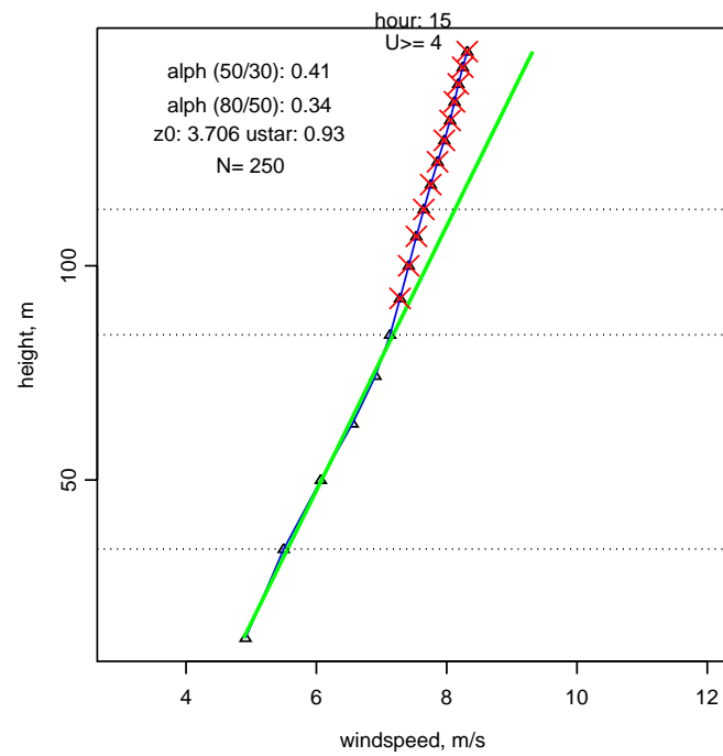
Figure 3 Mean wind profiles plotted with a logarithmic height axis for two different hours of the day. The straight line is the best straight-line fit for the profile below 80 m.
