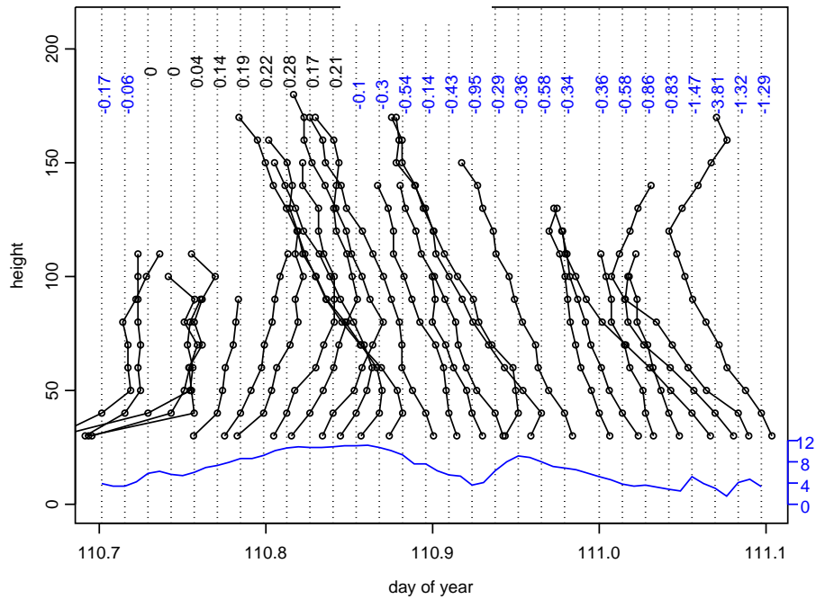
Figure 4 Time sequence of wind profiles during the night of April 20-21, 2005 at a site in the Great Plains. Numbers at the top represent the 80/60 shear for the 10 minute period represented. Negative shears are shown in blue. The blue line at the bottom depicts the mean wind speed at 50 m.
