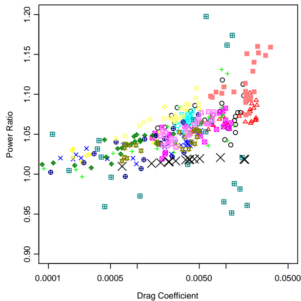
Figure 5 Power ratio for the 15 sites included in the study, plotted against the drag coefficient for each particular wind profile. Note that the drag coefficient is shown on a log scale. The black “X”s are the benchmark value of PR for each profile, assuming that a logarithmic profile applied throughout the rotor plane.
