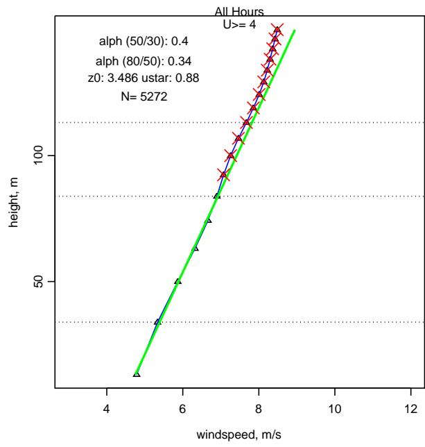
Figure 2 Two representations of the same average wind profile. (upper) with linear height axis and (lower) logarithmic height axis. Triangles are sodar measurements. Typical turbine rotor plane and hub height are denoted with horizontal dashed lines. The dashed line in the upper plot is the extrapolated power law profile using the 50/30 m shear parameter. In the lower plot, the logarithmic profile is defined by the best-fit straight line to the observations below 80 m. Observations that deviate from the logarithmic profile by more than 5% are denoted by red “X”s.
