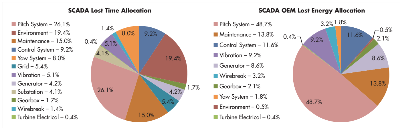
Figure 1: Health Monitoring – Energy To Downtime
